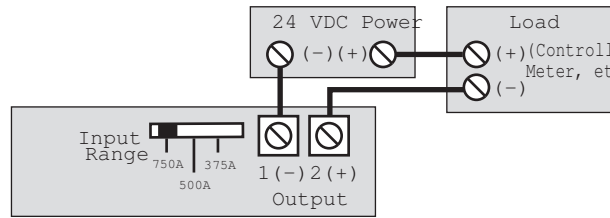
Single Transducer Installation
