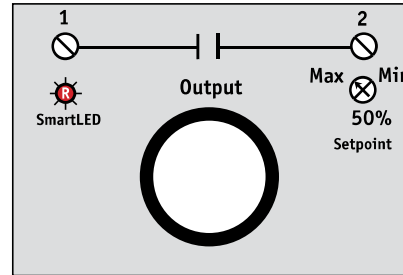
Solid-Core Connection
