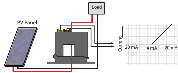
A typical photovoltaic panel monitoring connection.
