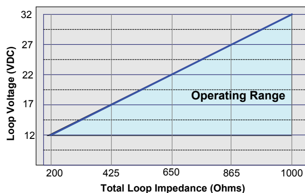
Maximum Loop Impedance
