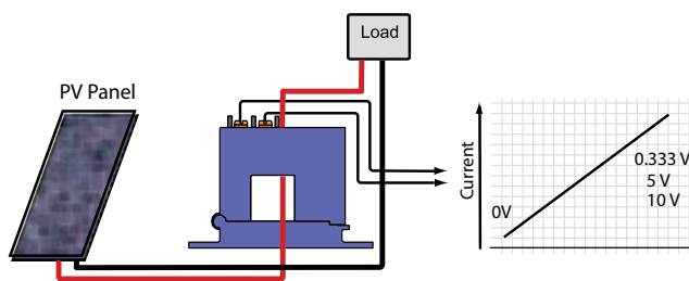
Photovoltaic Panel Output Measurement
